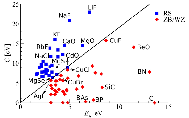
FIG. 1: Experimental ground-state structures of 68 octet binary compounds, arranged according to the two-dimensional descriptor introduced by Phillips and van Vechten [1, 2]. Because of visibility reasons, only 10 materials are labeled for each structure. See the SI for more details.
