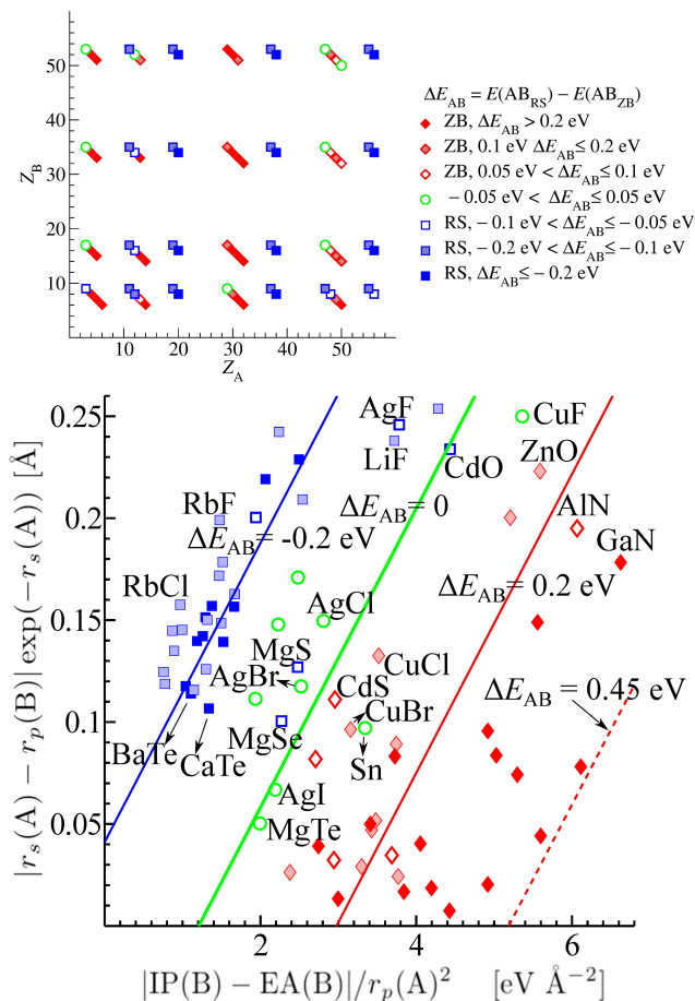
FIG. 2: Calculated energy differences between RS and ZB structures of the 82 octet binary AB materials, arranged by using the nuclear numbers ( Z_A, Z_B ) as descriptor (top) and according to our optimal two-dimensional descriptor (bottom). In the bottom panel, seven ZB materials with predicted \Delta E_{AB} > 0.5 eV are outside the shown window (see SI).
