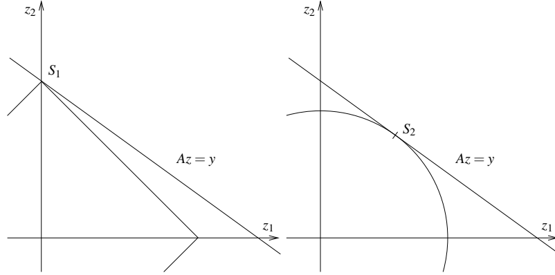
Fig. 1.2 Solution of S_p = \operatorname{argmin}_{z \in \mathbb{R}^2} \|z\|_p \quad \text{s.t.} \quad y = Az for p = 1 and p = 2
