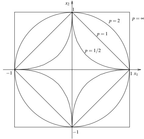
Fig. 1.1 Shape of the l_p^2 unit ball for p = 1/2, p = 1, p = 2 and p = \infty
