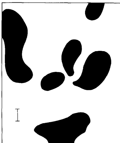
Figure 2. An example of a "dappled" pattern as resulting from a type (a) morphogen system. A marker of unit length is shown (see text, Sections 9 and 11).
