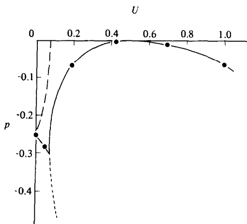
Figure 1. Values of \mathcal{R}p (instability or growth rate), and |\mathcal{I}p| (radian frequency of oscillation), related to wavelength 2\pi U^{-1/2} as in the relation (18) with I=0 . This is a case of stationary waves with finite wavelength. Full line, \mathcal{R}p ; broken line, -|\mathcal{I}p| (zero for U > 0.071 ); dotted line, \mathcal{R}p' . The full circles on the curve for \mathcal{R}p indicate the values of U, p actually achievable on the finite ring considered in Section 10, with s=0 on the extreme left, s=5 on the right.
