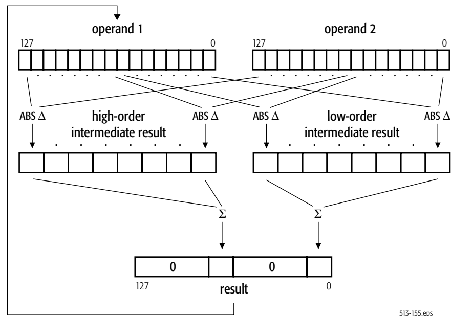
Figure 4-9. Sum-of-Absolute-Differences Operation
