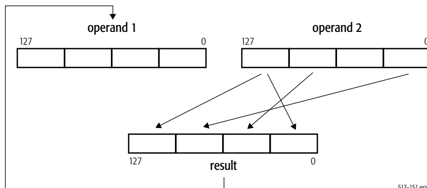
Figure 4-5. Shuffle Operation
