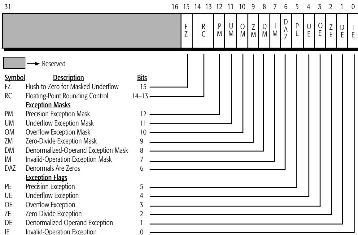
Figure 4-13. 128-Bit Media Control and Status Register (MXCSR)
