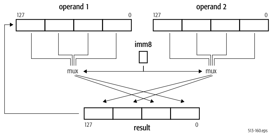
Figure 4-34. SHUFPS Shuffle Operation
