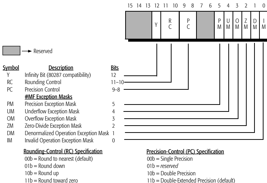
Figure 6-4. x87 Control Word Register (FCW)
