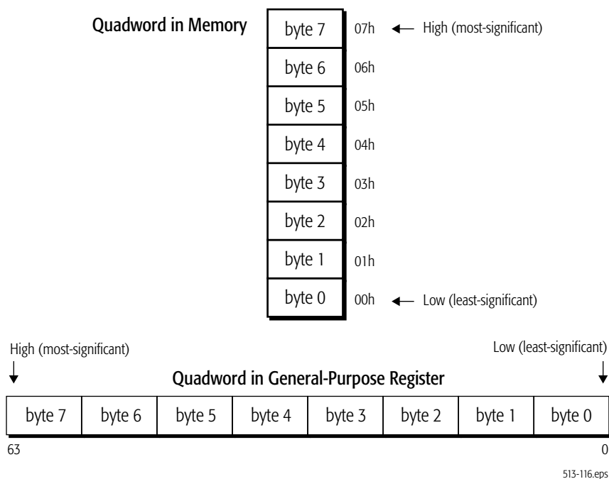
Figure 2-5. Byte Ordering
