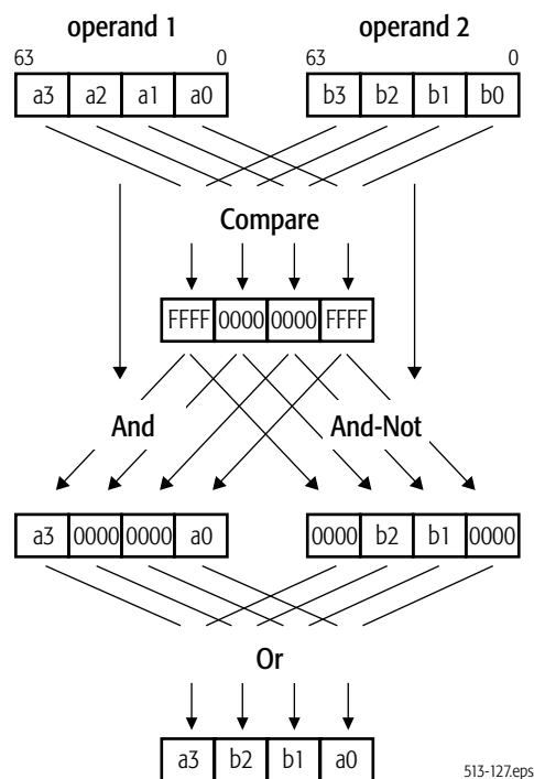
Figure 5-5. Branch-Removal Sequence
