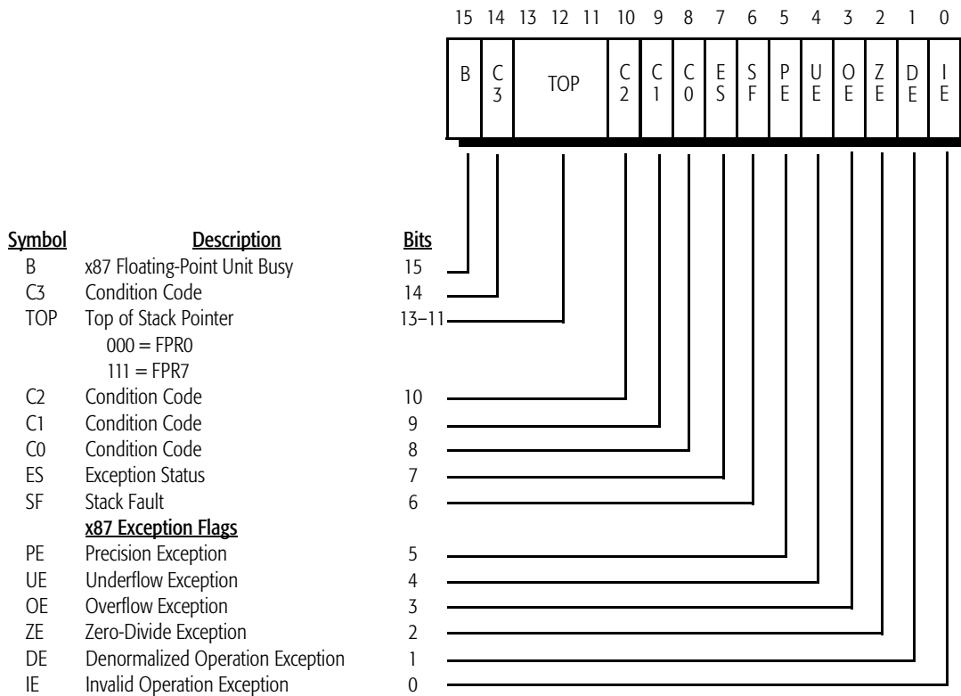
Figure 6-3. x87 Status Word Register (FSW)
