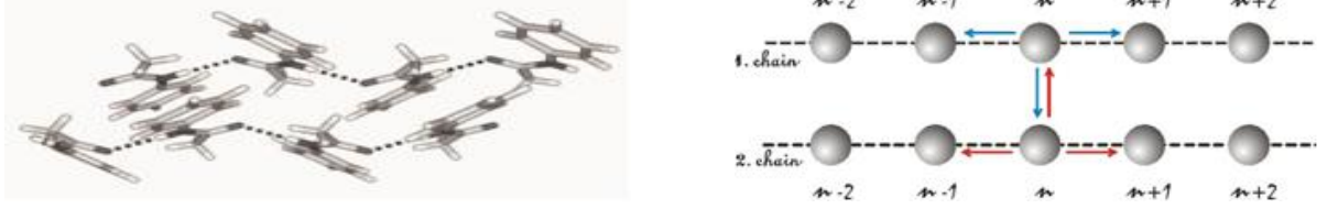
Figure 1. The real structure of the part of crystalline acetanilide macromolecular chains is shown in the left, whereas its schematic structure is demonstrated in the right. The possible vibron hopping transitions are shown by the arrows.
