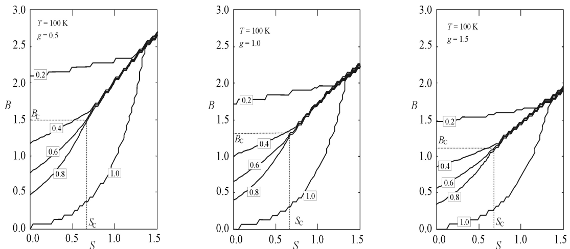
Figure 2. The dependence of the variational parameter \delta on the system parameters S , B , g at T = 100 K.
